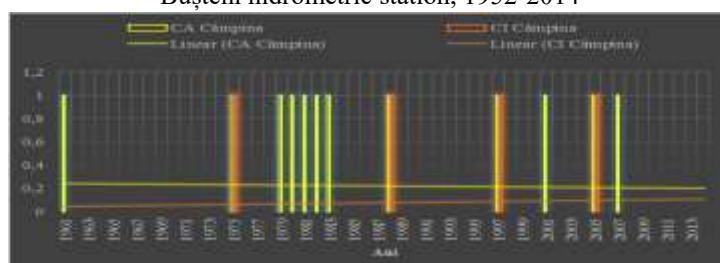
Fig. 8 – The number of annual events of overcoming the Warning and Flood Levels at Câmpina hidrometric station, 1961-2014
