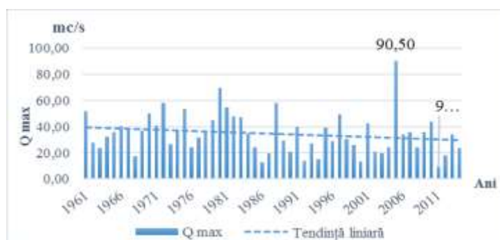
Fig. 3 – Annual maximum flow at Câmpina hydrometric station (1961-2014)
