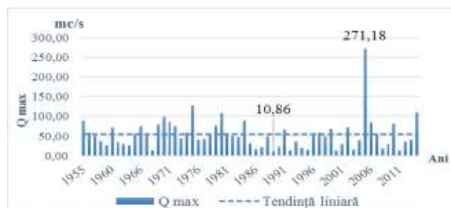
Fig. 4 – Annual maximum flow at Moara Domnească hydrometric station (1955-2014)
