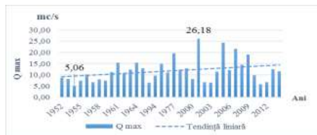
Fig. 2 – Annual maximum flow at Bușteni hydrometric station (1952-2014)
