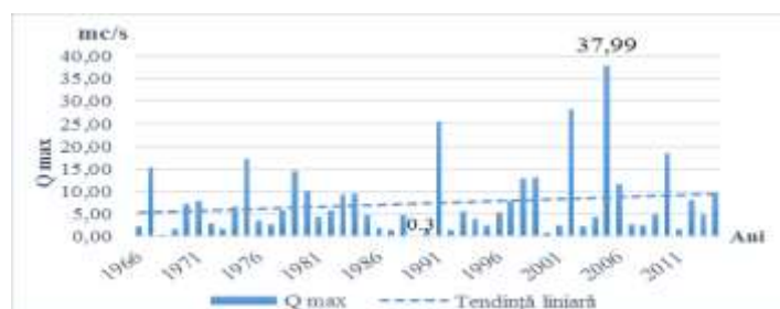
Fig. 5 – Annual maximum flow at Vărbilau hydrometric station (1966-2014)
